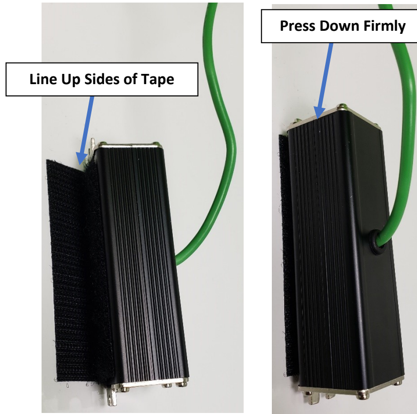
Figure 10 - Line Up and Attach Suppressor (Ready to Ground)
