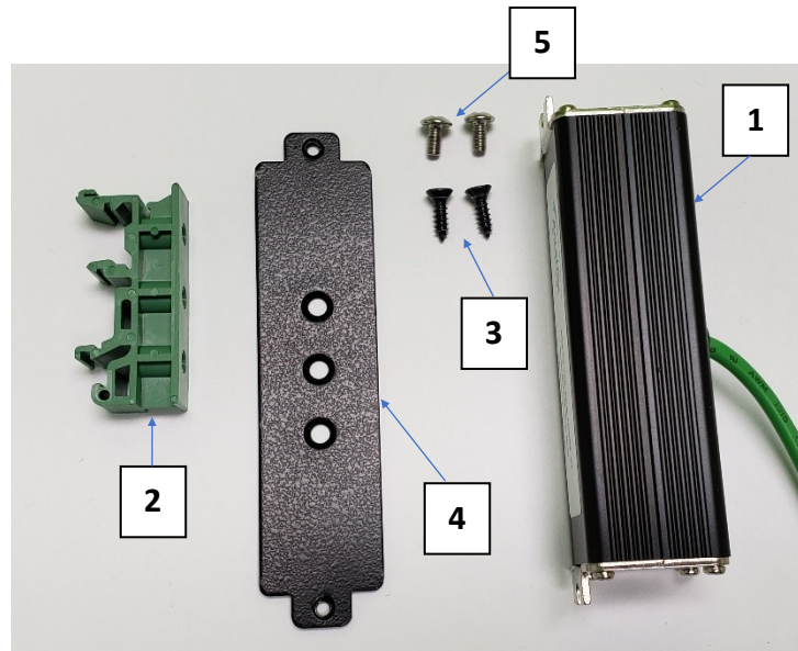
Figure 1 - Parts Required for DIN Rail Install
