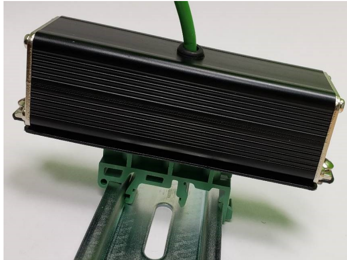
Figure 6 - Attached to DIN Rail (Ready to Ground)
