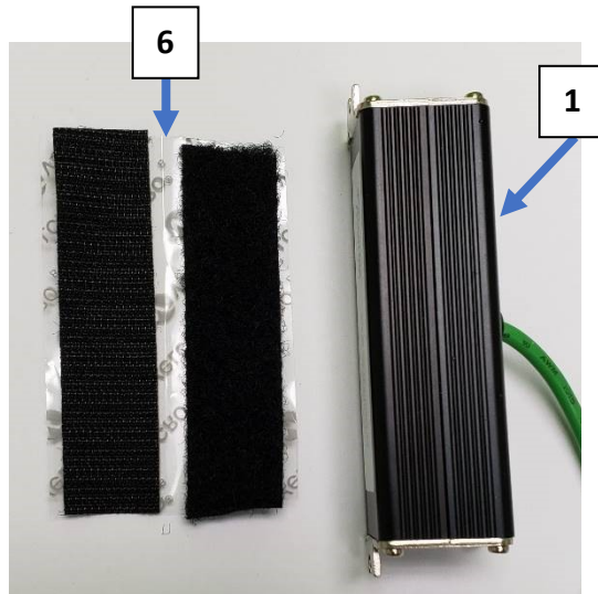
Figure 7 - Parts Required for Velcro tape Install
