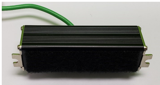
Figure 9 - Attach Velcro Tape to Bottom of Suppressor
