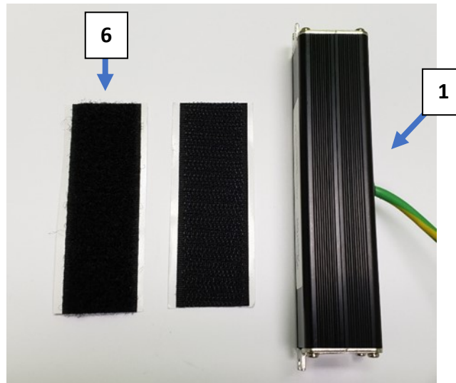
Figure 7 - Parts Required for Velcro tape Install
