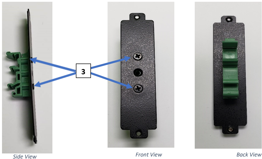
Figure 2 - DIN Rail Clip to DIN Rail Attachment Bar
